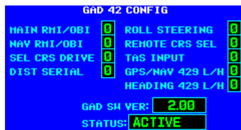
Figure 5-23. GAD 42 CONFIG Page
